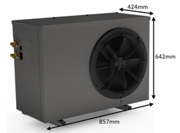
Outside unit
